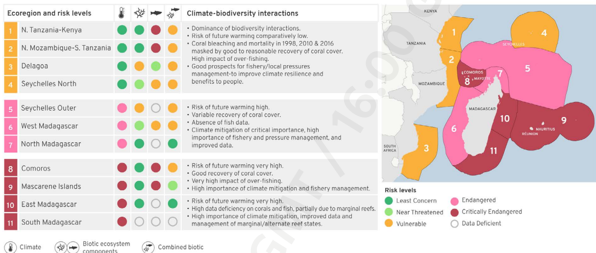
Figure 5. Ecoregions of the Western Indian Ocean showing their risk of coral reef collapse in the IUCN Red List of Ecosystems. 6 Risk levels for climate (thermometer icon) and biotic (coral and fish icons) ecosystem components are shown with their individual levels of risk. The combined biotic risk level is shown in the ring around the coral/fish icons, and for each ecoregion by background shading and the map. The text highlights biodiversity-climate interactions, prospects for management and benefits for people.
